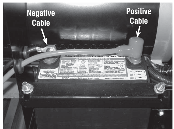
Figure 3 - Battery Connections
